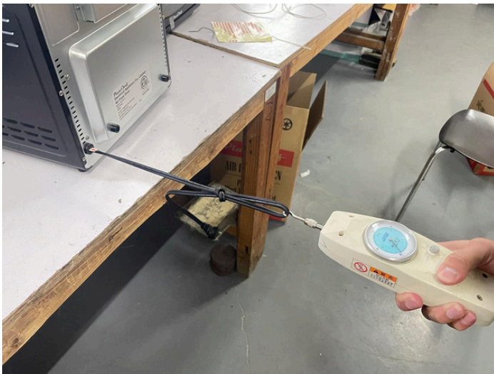
Pull test on power cord
